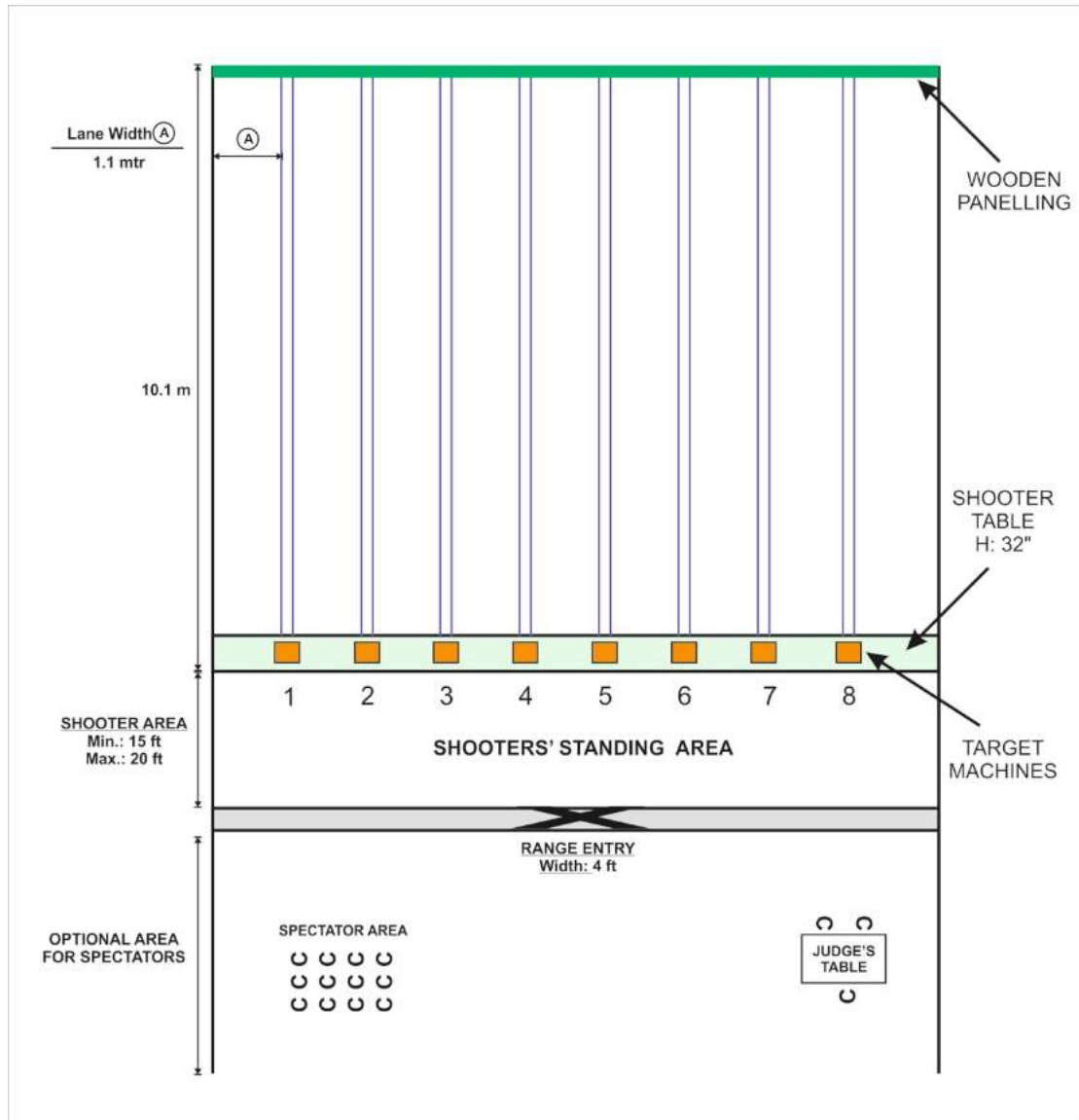
Typical Layout of an 8-lane, 10m Shooting Range
